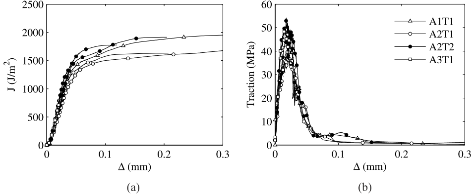
Figure 4.9: J vs. crack tip opening and shear displacements norm (a) and measured cohesive laws (b) of the MMB 50% tests conducted. Only 1 out of every 100 points is depicted for clarity.
