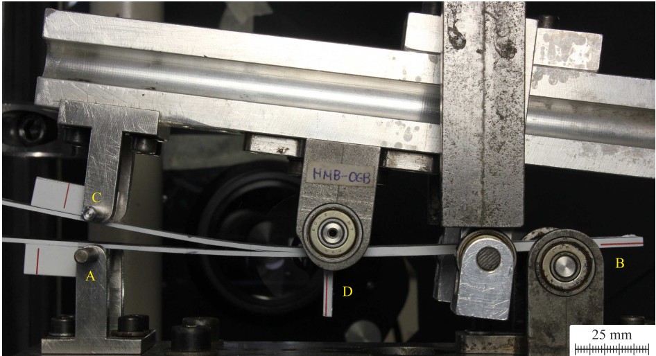
Figure 2.3: Picture taken during the test used for the angle measurement.
