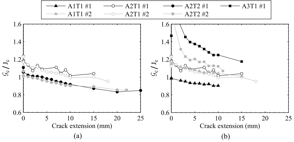
Figure 3.7: Effect of the adhesive (a) and adherend (b) thicknesses on the relative difference between \mathcal{G}_c and J_c for DCB tests.
