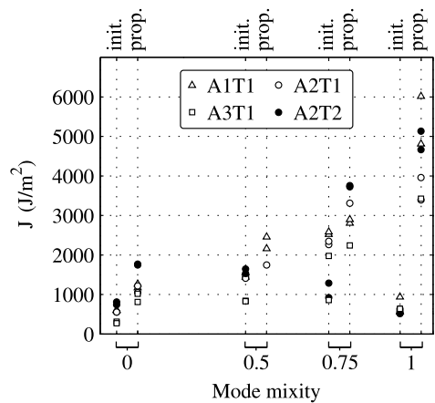
Figure 4.6: Summary of the initiation and propagation fracture toughness values obtained as a function of the aimed mode mixity.
