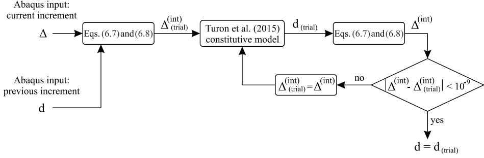
Figure 6.3: Iterative procedure for the computation of the interface displacement jumps.
