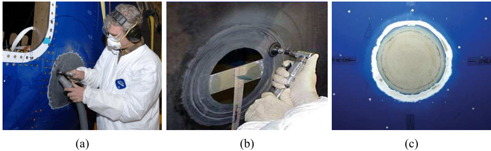
Figure 1.2: Damage repair in an aircraft structure ( source: The Boeing Co. ).
