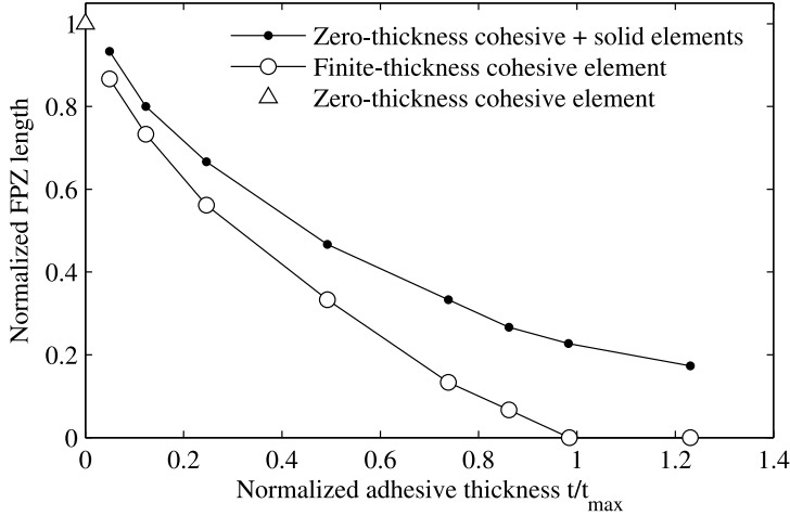
Figure 6.6: FPZ length as a function of the adhesive thickness for the DCB test.
