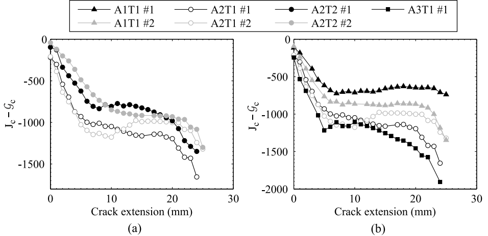
Figure 3.5: Effect of the adhesive (a) and adherend (b) thicknesses on the absolute difference between \mathcal{G}_c and J_c for ENF tests.
