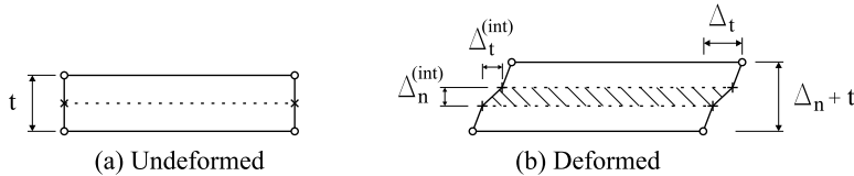
Figure 6.2: Schematic representation of the decoupling between the bulk adhesive and the embedded interface in an a) undeformed and b) deformed state.
